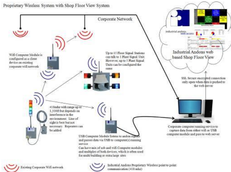
Proprietary Wireless System with Shop Floor View System
